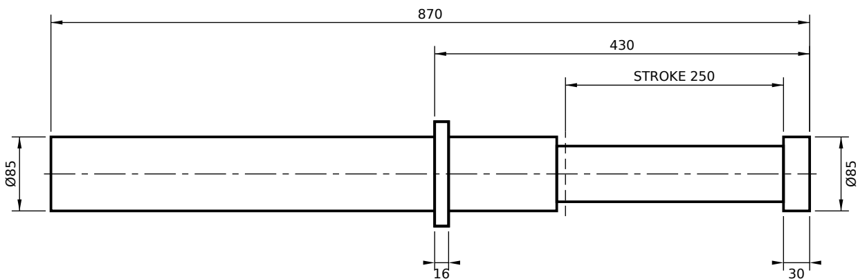
FRONT FLANGE MOUNT (FS)
