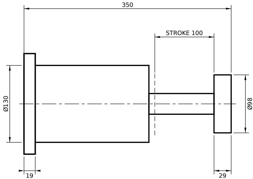
REAR FLANGE MOUNT (RS)
