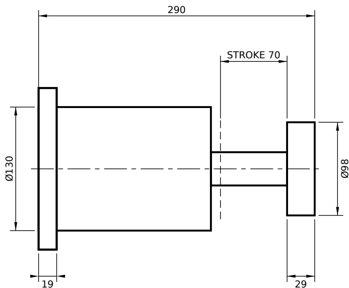
REAR FLANGE MOUNT (RS)
