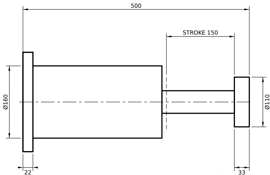
REAR FLANGE MOUNT (RS)
