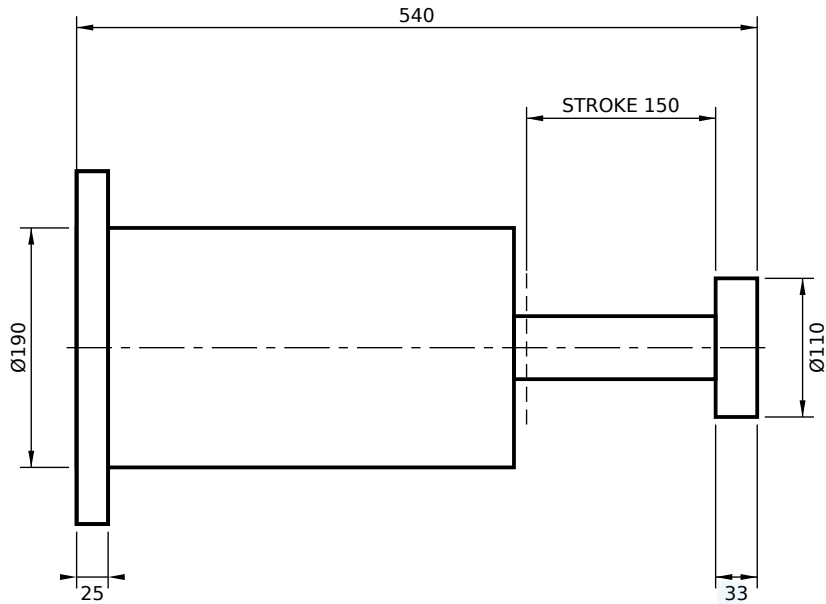
REAR FLANGE MOUNT (RS)
