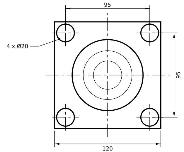
VIEW FROM ROD END (SCALE 1:2.5)
