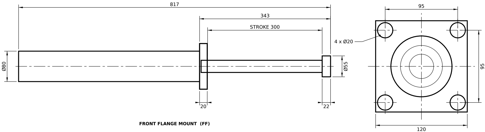
VIEW FROM ROD END (SCALE 1:2.5)
