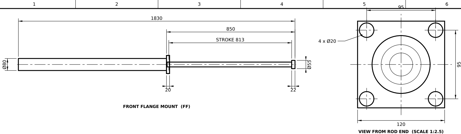
VIEW FROM ROD END (SCALE 1:2.5)
