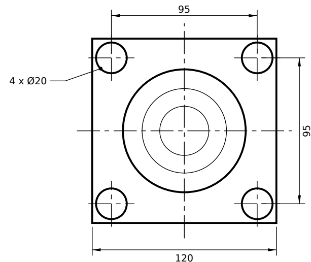
VIEW FROM ROD END (SCALE 1:2.5)
