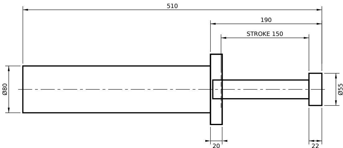
FRONT FLANGE MOUNT (FF)
