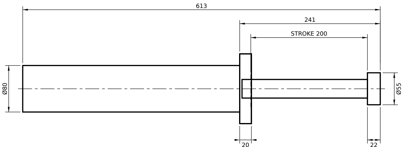
FRONT FLANGE MOUNT (FF)
