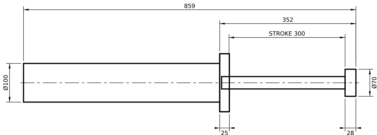
FRONT FLANGE MOUNT (FF)
