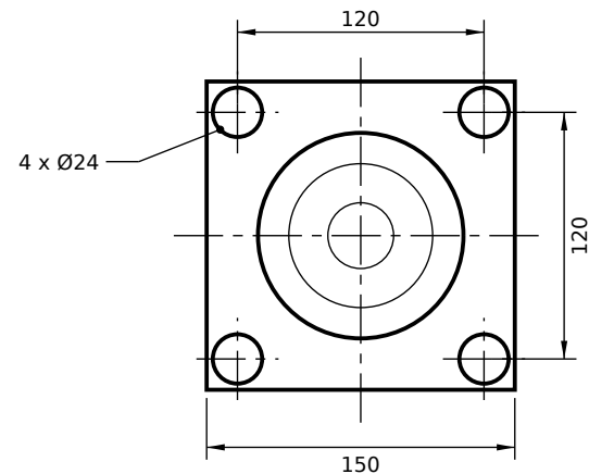
VIEW FROM ROD END (SCALE 1:4)
