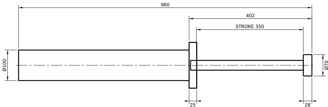
FRONT FLANGE MOUNT (FF)
