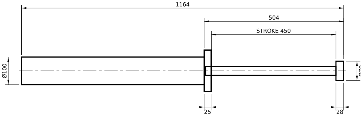
FRONT FLANGE MOUNT (FF)
