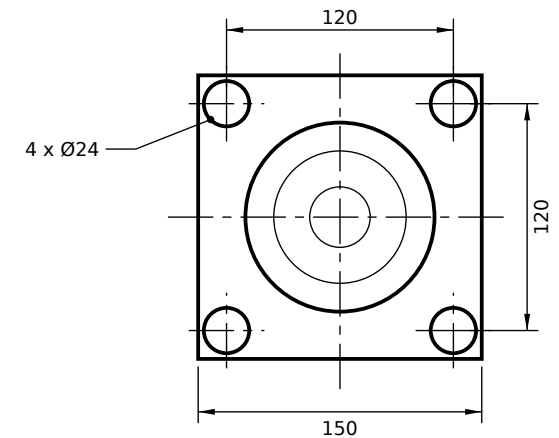
VIEW FROM ROD END (SCALE 1:4)
