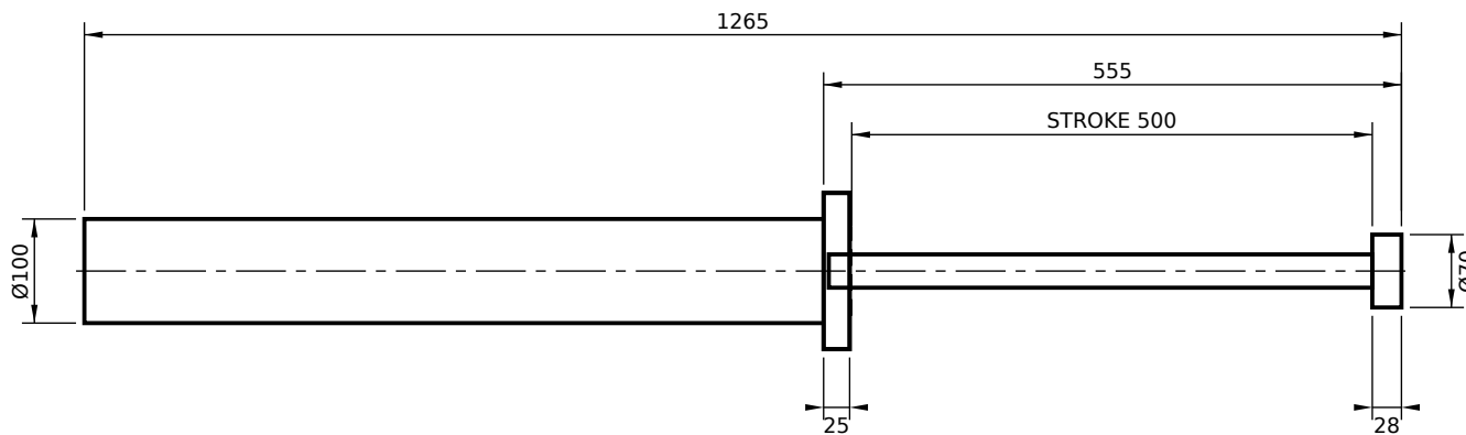
FRONT FLANGE MOUNT (FF)
