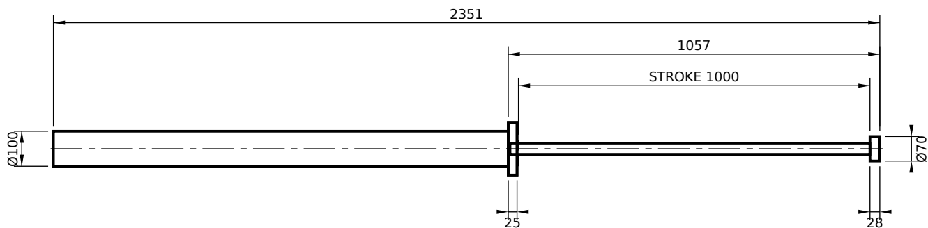
FRONT FLANGE MOUNT (FF)
