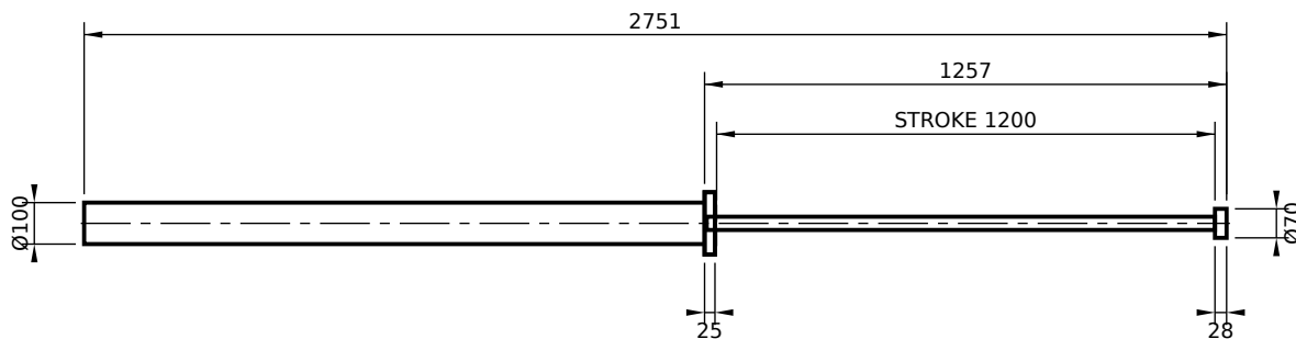
FRONT FLANGE MOUNT (FF)
