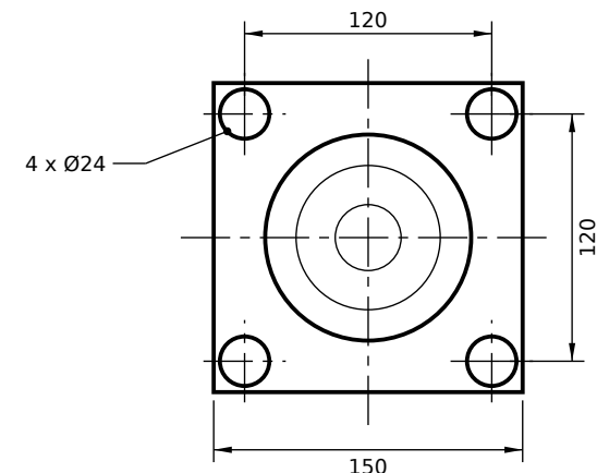
VIEW FROM ROD END
