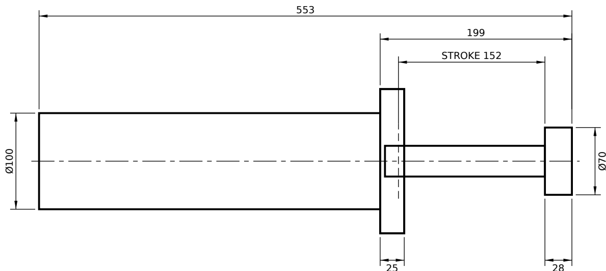
FRONT FLANGE MOUNT (FF)
