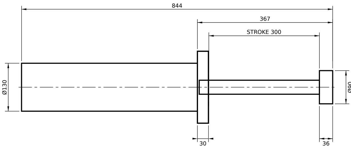
FRONT FLANGE MOUNT (FF)
