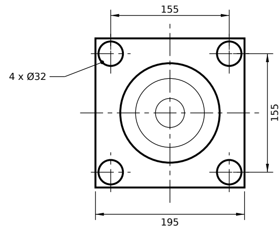
VIEW FROM ROD END (SCALE 1:5)
