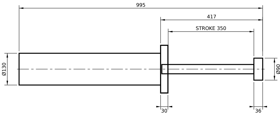
FRONT FLANGE MOUNT (FF)
