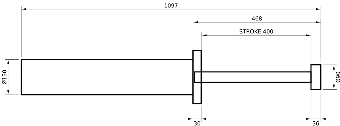
FRONT FLANGE MOUNT (FF)
