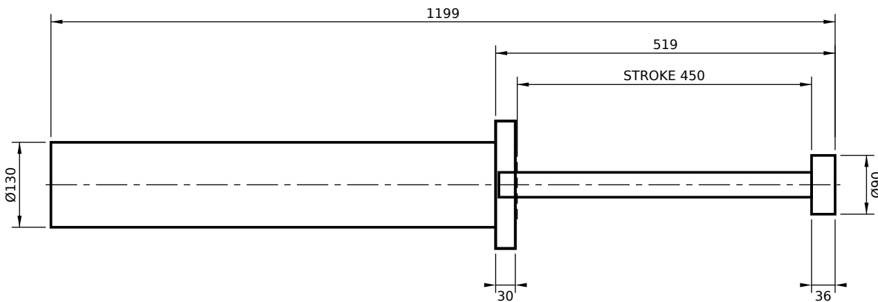
FRONT FLANGE MOUNT (FF)
