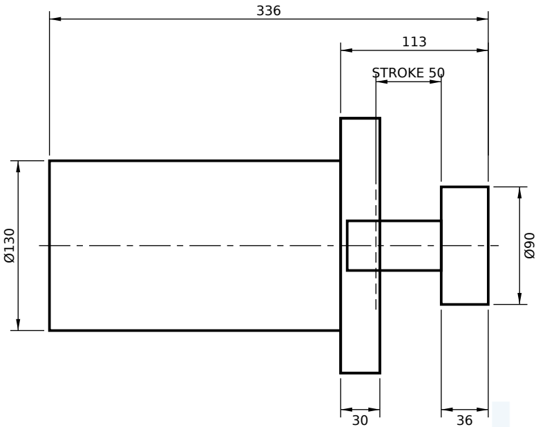
FRONT FLANGE MOUNT (FF)
