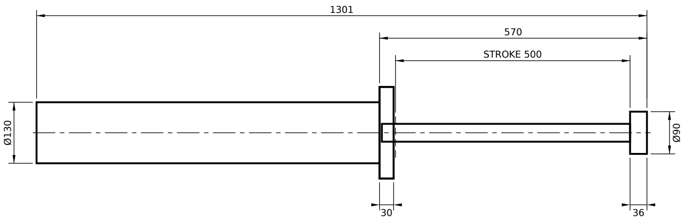
FRONT FLANGE MOUNT (FF)
