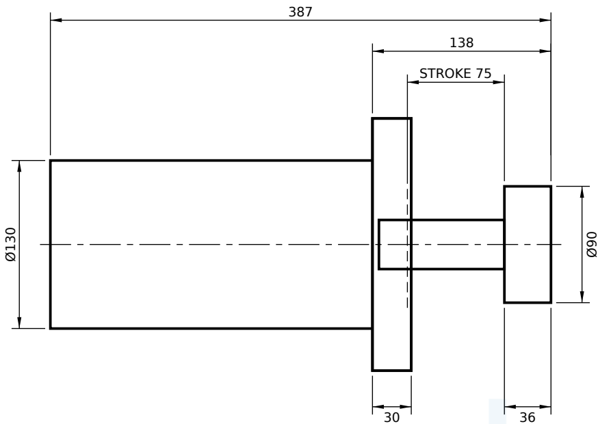
FRONT FLANGE MOUNT (FF)
