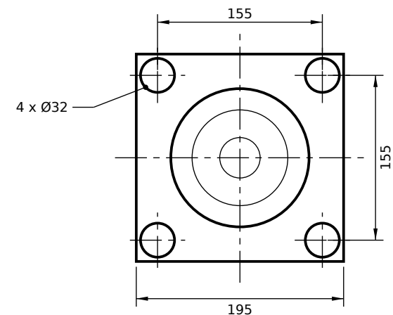
VIEW FROM ROD END (SCALE 1:5)
