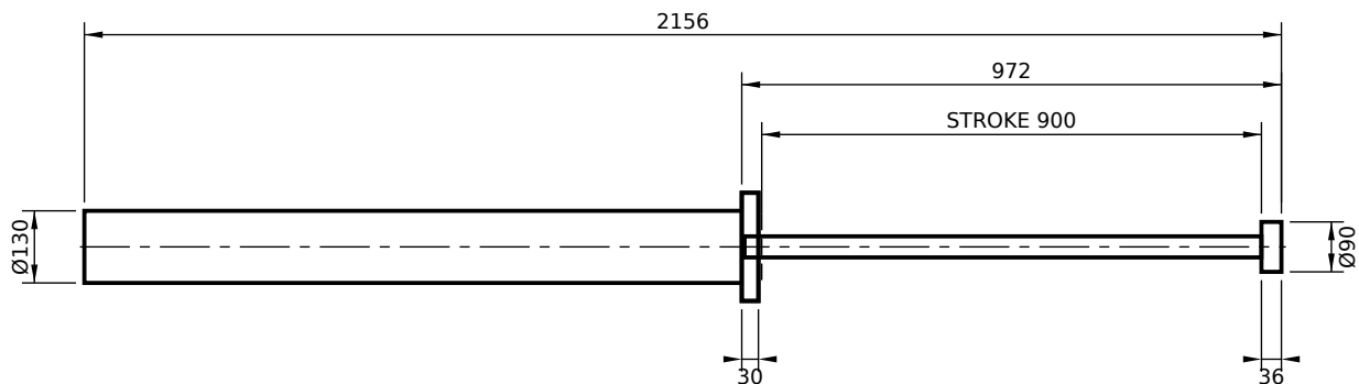
FRONT FLANGE MOUNT (FF)
