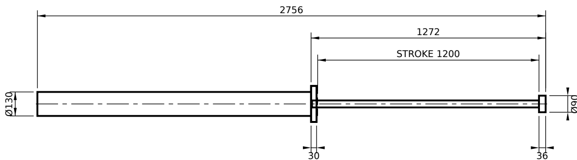
FRONT FLANGE MOUNT (FF)
