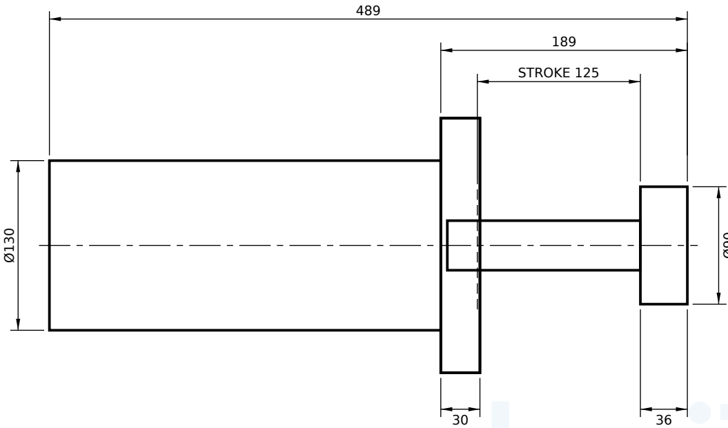
FRONT FLANGE MOUNT (FF)
