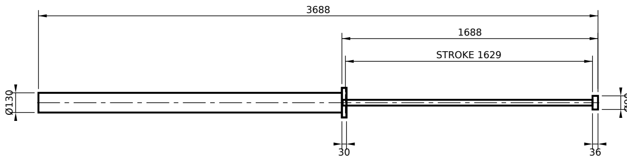
FRONT FLANGE MOUNT (FF)
