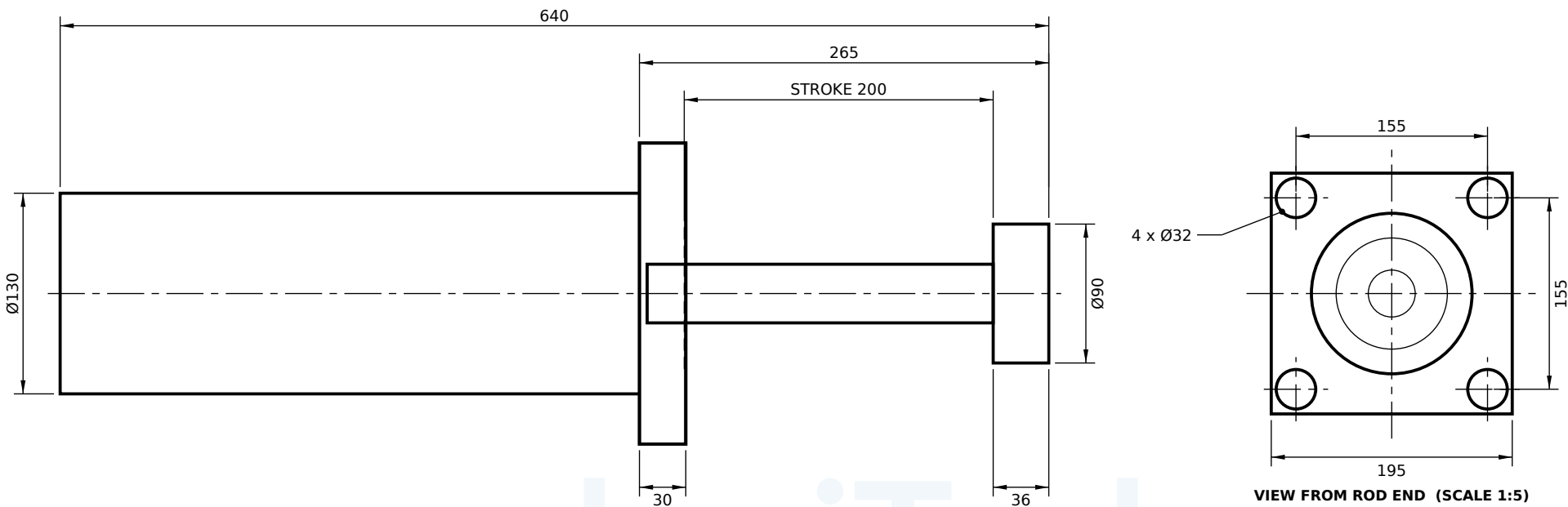
FRONT FLANGE MOUNT (FF)
