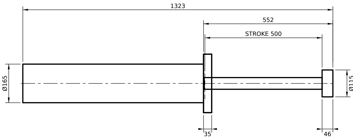
FRONT FLANGE MOUNT (FF)
