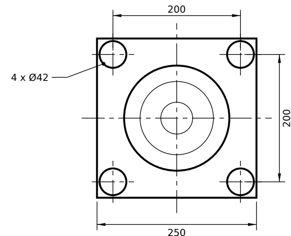
VIEW FROM ROD END (SCALE 1:6)
