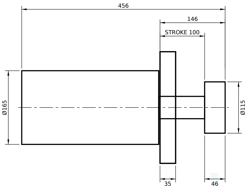
FRONT FLANGE MOUNT (FF)
