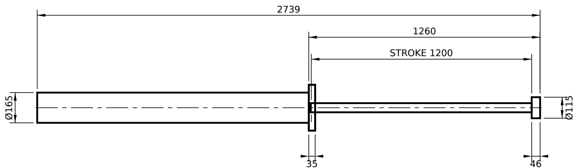
FRONT FLANGE MOUNT (FF)
