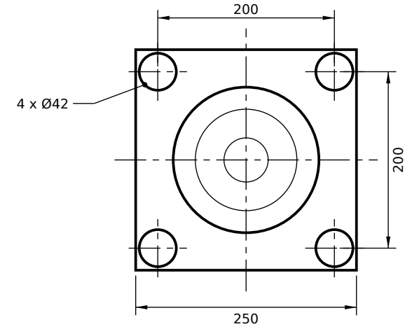
VIEW FROM ROD END (SCALE 1:6)
