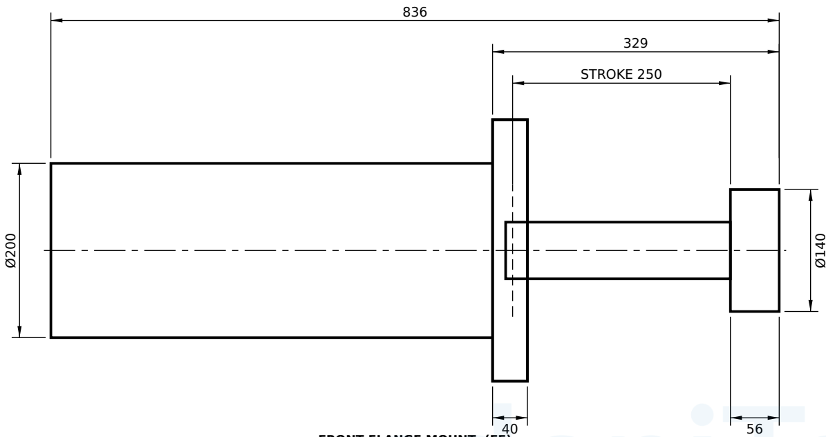
FRONT FLANGE MOUNT (FF)
