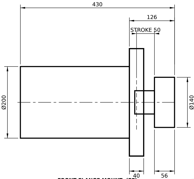
FRONT FLANGE MOUNT (FF)
