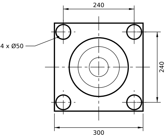
VIEW FROM ROD END (SCALE 1:8)
