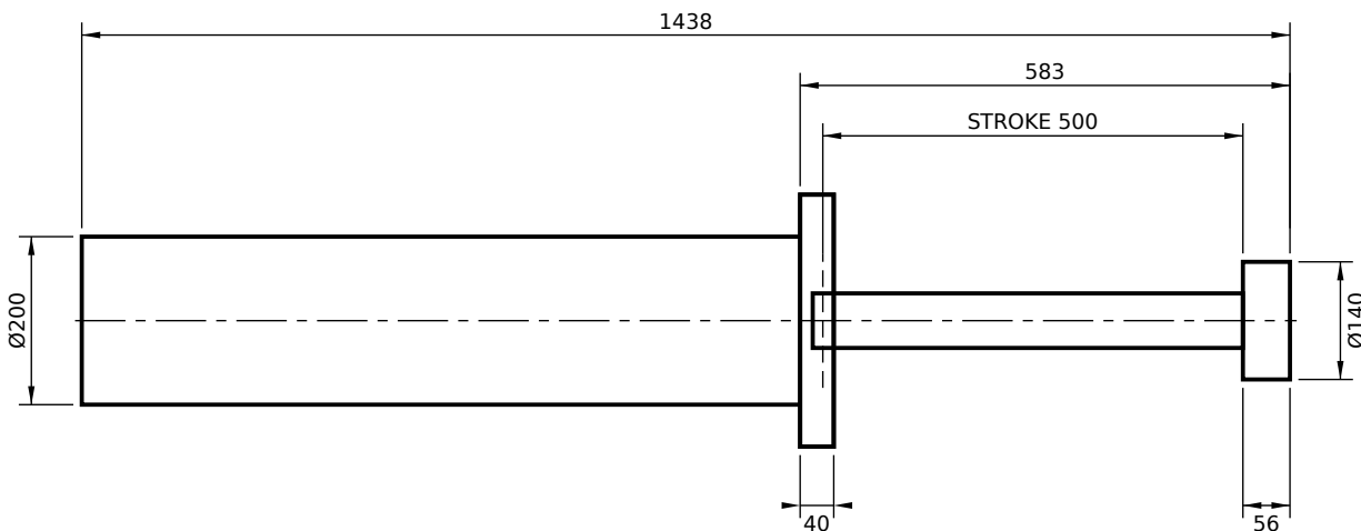
FRONT FLANGE MOUNT (FF)
