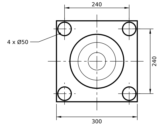
VIEW FROM ROD END (SCALE 1:8)
