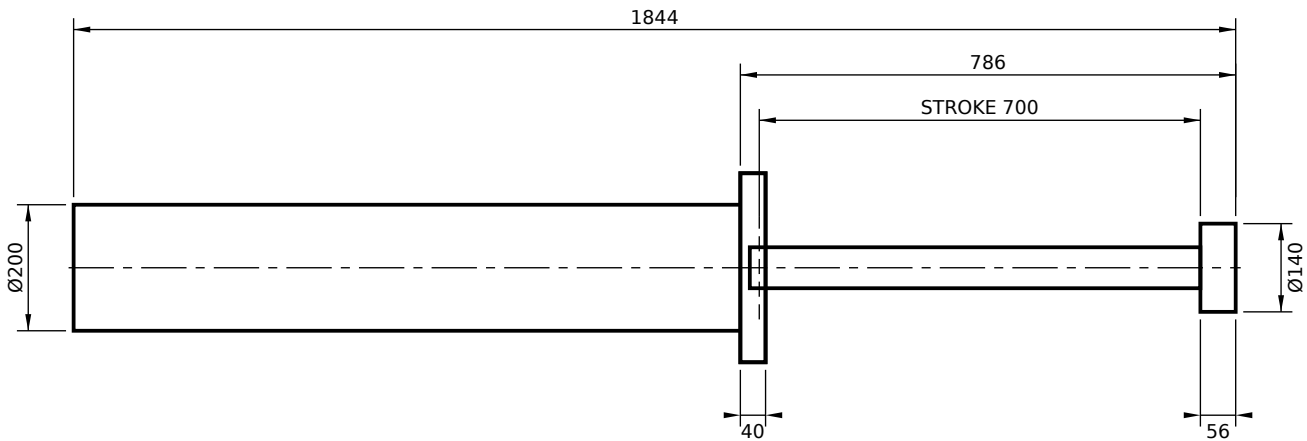
FRONT FLANGE MOUNT (FF)
