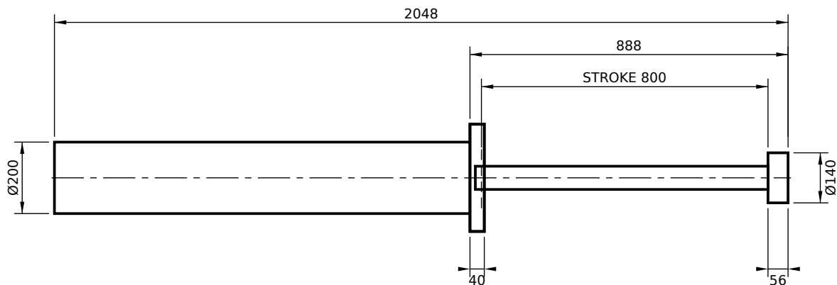
FRONT FLANGE MOUNT (FF)
