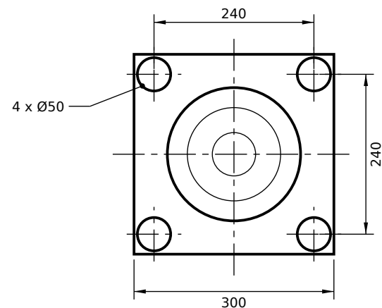
VIEW FROM ROD END (SCALE 1:8)
