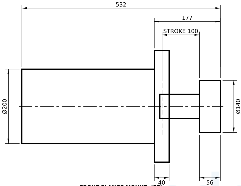
FRONT FLANGE MOUNT (FF)
