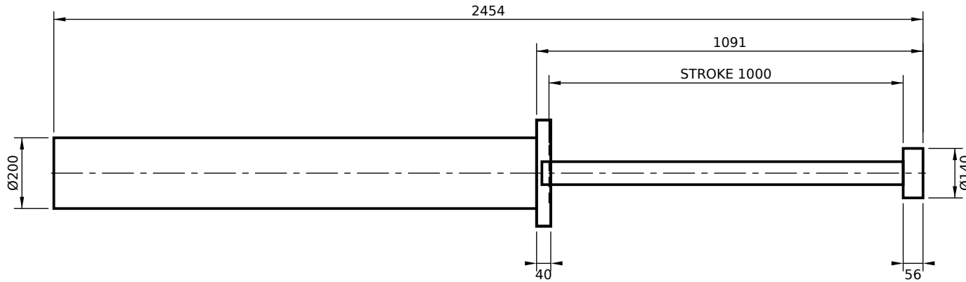
FRONT FLANGE MOUNT (FF)
