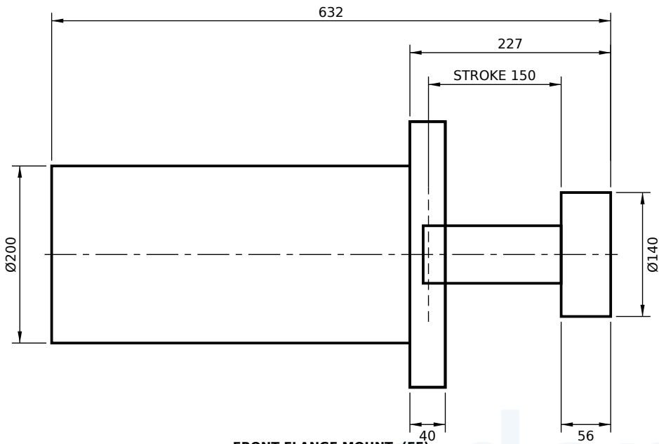
FRONT FLANGE MOUNT (FF)
