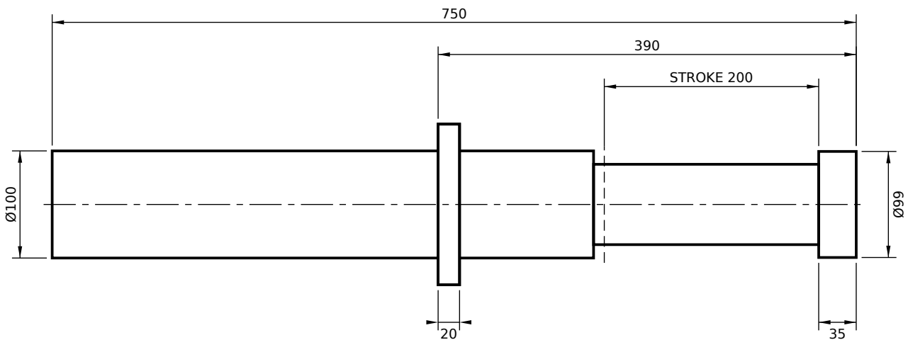
FRONT FLANGE MOUNT (FF)
