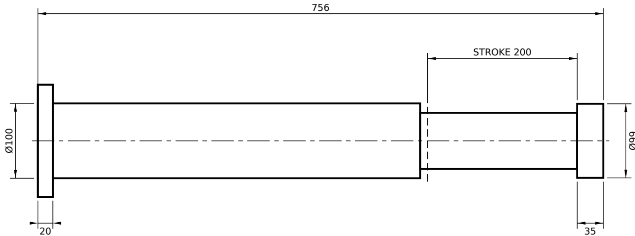
REAR FLANGE MOUNT (FR)
