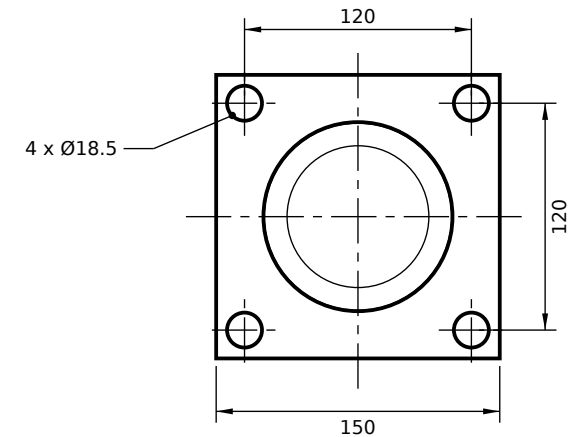
VIEW FROM ROD END (SCALE 1:4)
