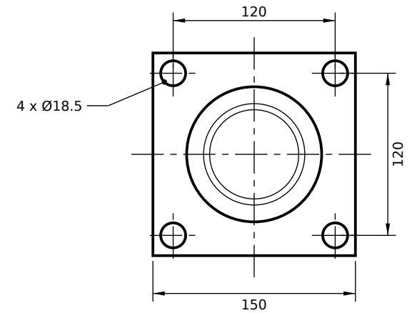
VIEW FROM ROD END (SCALE 1:4)
