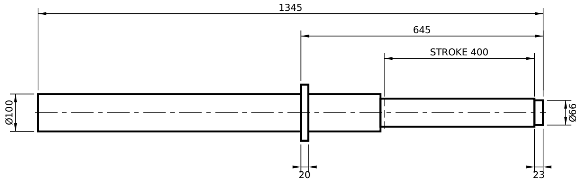
FRONT FLANGE MOUNT (FF)
