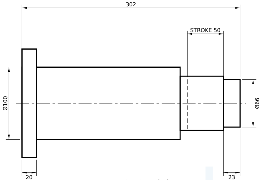
REAR FLANGE MOUNT (FR)
