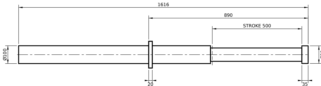
FRONT FLANGE MOUNT (FF)
