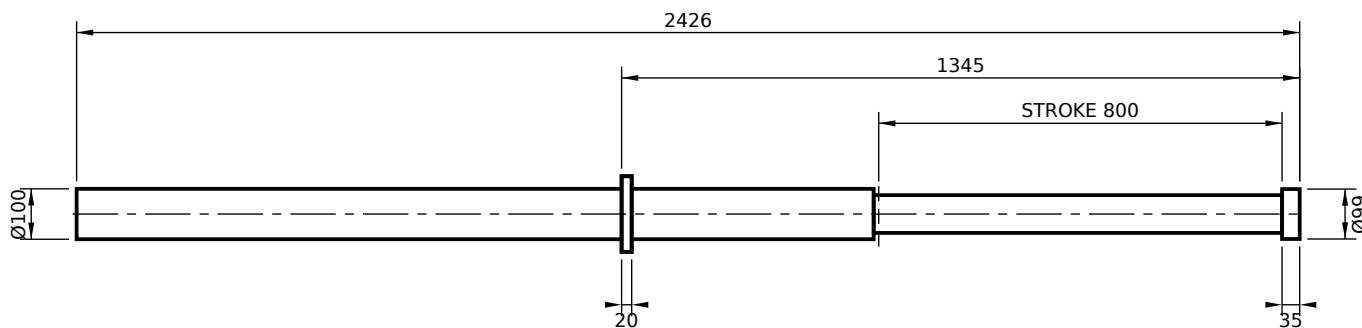
FRONT FLANGE MOUNT (FF)
