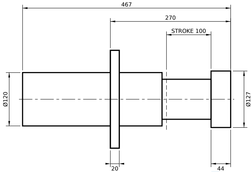
FRONT FLANGE MOUNT (FF)
