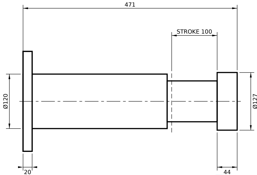
REAR FLANGE MOUNT (FR)
